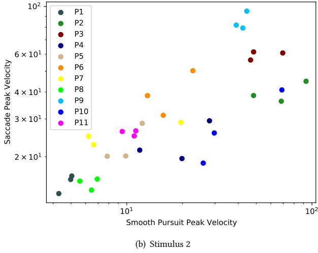
Figure 2: Visualization of the KNN that classifies the user’s identities for both stimuli. For better visibility, we only depict the smooth pursuit and saccade peak velocities (px/deg) on a log scale.
