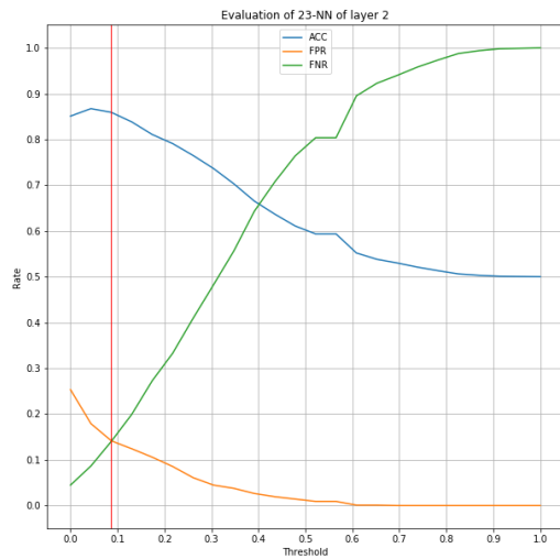
Figure 5: Determination of the EER and the corresponding threshold for layer 2 using k = 23 . The ACC, FPR, and FNR are calculated for every possible threshold. The red vertical line represents the threshold that yields the EER.
