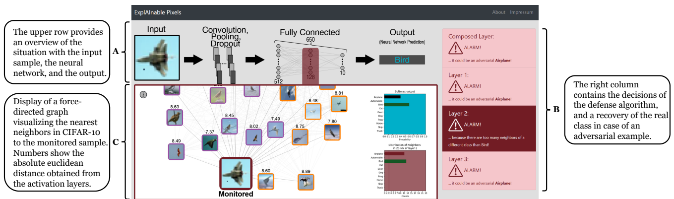
Figure 1: The “ExplAInable Pixels” web interface provides insights into deep learning models during adversarial attacks.
