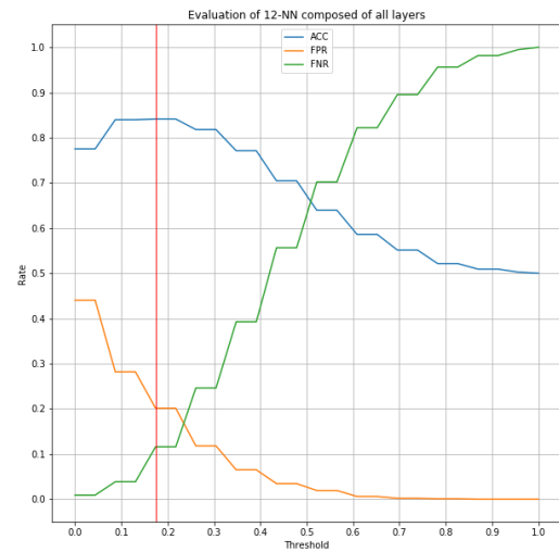
Figure 7: Determination of the EER and the corresponding threshold for the composed layer using k = 12 . The ACC, FPR, and FNR are calculated for every possible threshold. The red vertical line represents the threshold that yields the EER.
