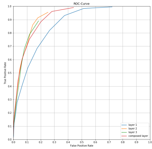
Figure 12: Comparison of the ROC curves across layers 1, 2, 3, and the composed layer using k = (13, 23, 12, 12) respectively. By varying the threshold for each layer, the FPR and TPR can be measured and plotted to show the trade-off and evaluate the quality of the defense algorithm per layer.
