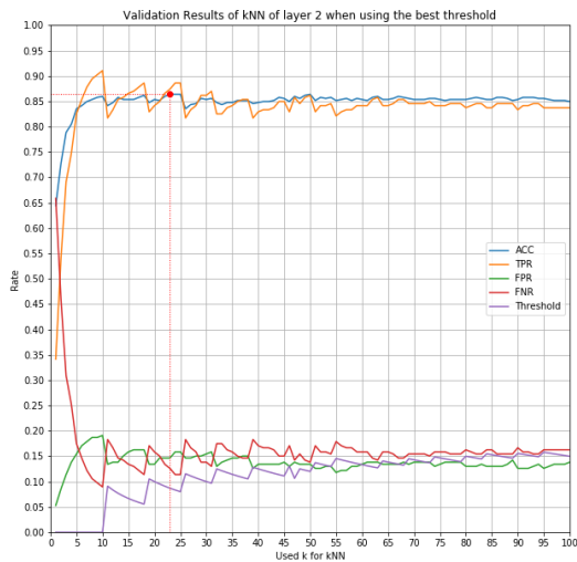
Figure 9: Determination of the best value for k and the corresponding best threshold for layer 2. For every k , the corresponding threshold meeting the EER is calculated. The validation results show that the highest accuracy can be achieved using k = 23 for layer 2 (red dashed line).
