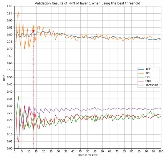
Figure 8: Determination of the best value for k and the corresponding best threshold for layer 1. For every k , the corresponding threshold meeting the EER is calculated. The validation results show that the highest accuracy can be achieved using k = 13 (red dashed line).
